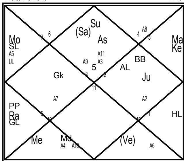
Natal Chart
