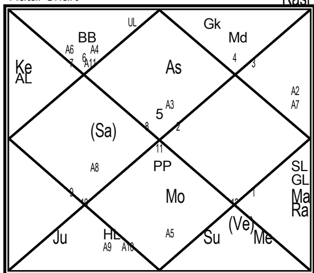
Natal Chart
